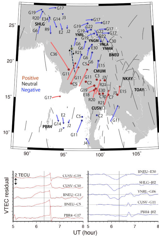
Fig.1. (top) Sub-ionospheric point (300 km altitude) trajectories of GNSS satellites from 11 ground stations showing positive (red), negative (blue), and no (black) anomalies. (bottom) VTEC residual plots for various ground stations over time (UT hour).
