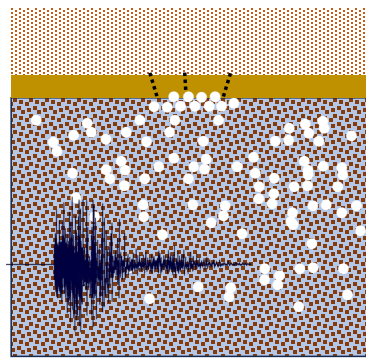
Degassing induced by seismic shaking (Champagne effect)
